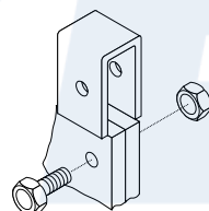
CLIP DETAIL
