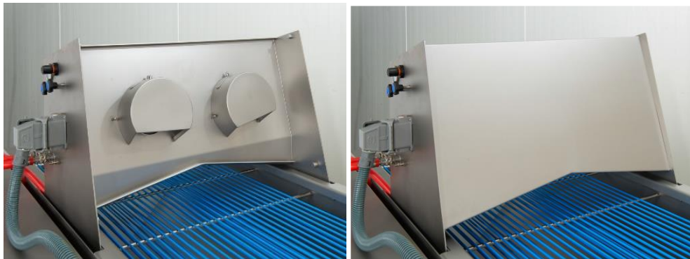
Example of a dischood with 2 discs
