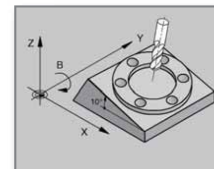
Tilting working plane
