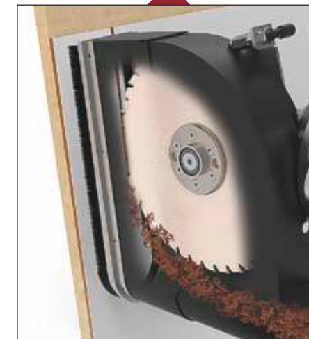
HPL CUT
