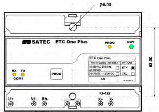
Figure 2-2 Surface mounting
