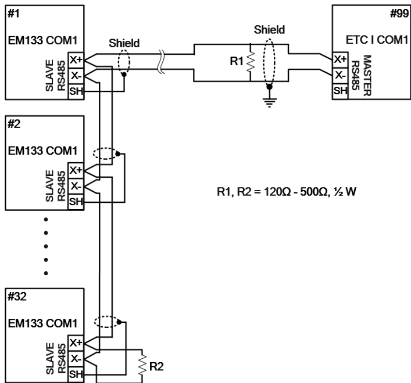
Figure 2-6 COM1 RS-485 2-Wire Connection
