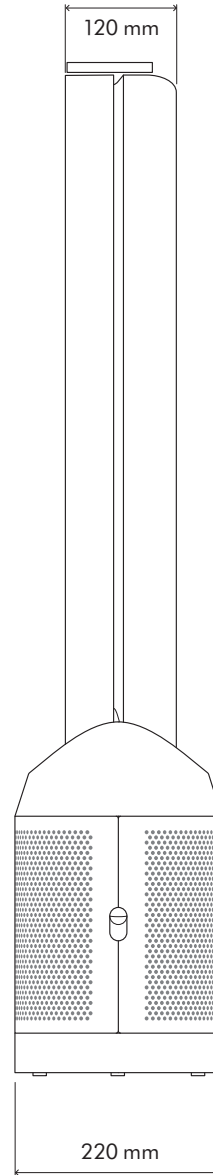
Side elevation
