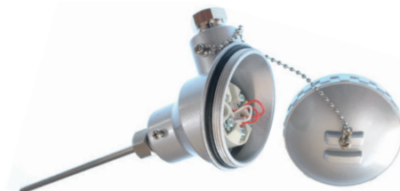
C Platinum Resistance Pt100 3 wire class B Resistance Thermometer with KNE Head and Fitted Transmitter
