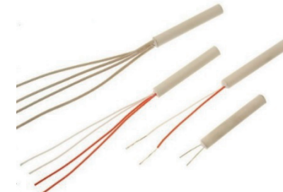
Pt100 Tubular Ceramic Insert Elements with tail wires
