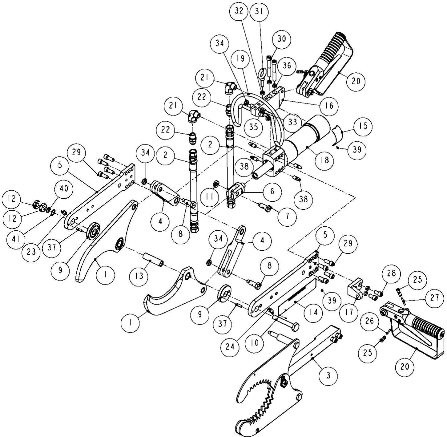
Figure 2 MODEL "HC-3" – MAIN ASSEMBLY
