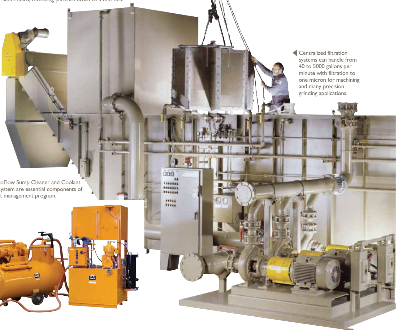
▲ Eriez HydroFlow SumpDoc™ removes metal chips as well as completely filters fluids, removing particles down to 5 microns.
