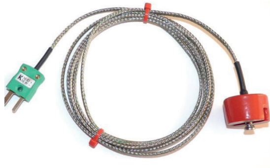
A Magnet Thermocouple
