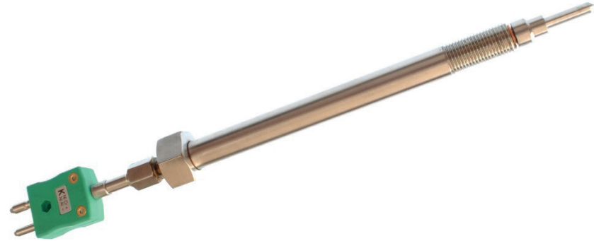
B Twist Melt Bolt Thermocouple with Standard Thermocouple Plug
