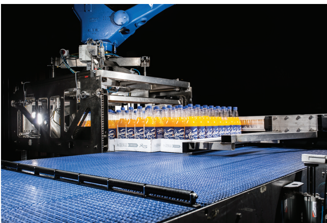
The automatic pusher for multipack is fully integrated in the MOTOMAN robot's control system.
