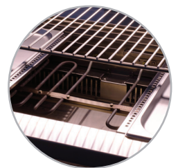
Heating element above water tray for humidification
