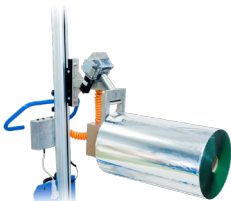
Pneumatic expander
