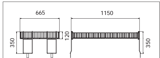
TA9-665P table platform: weight 8 kg
