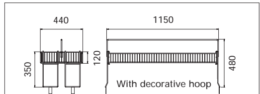
TA9-440P table platform: weight 6 kg
