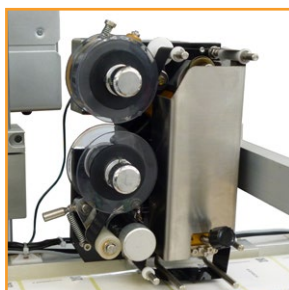
Hot foil coding units
