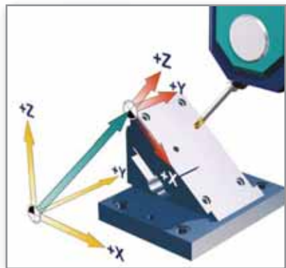
Swivel (CYCLE 800)
