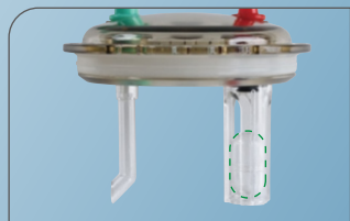
The capsule shaped floating control may fully prevent overflow by any angles. The angle pipe may lead the fluid in fluently.
