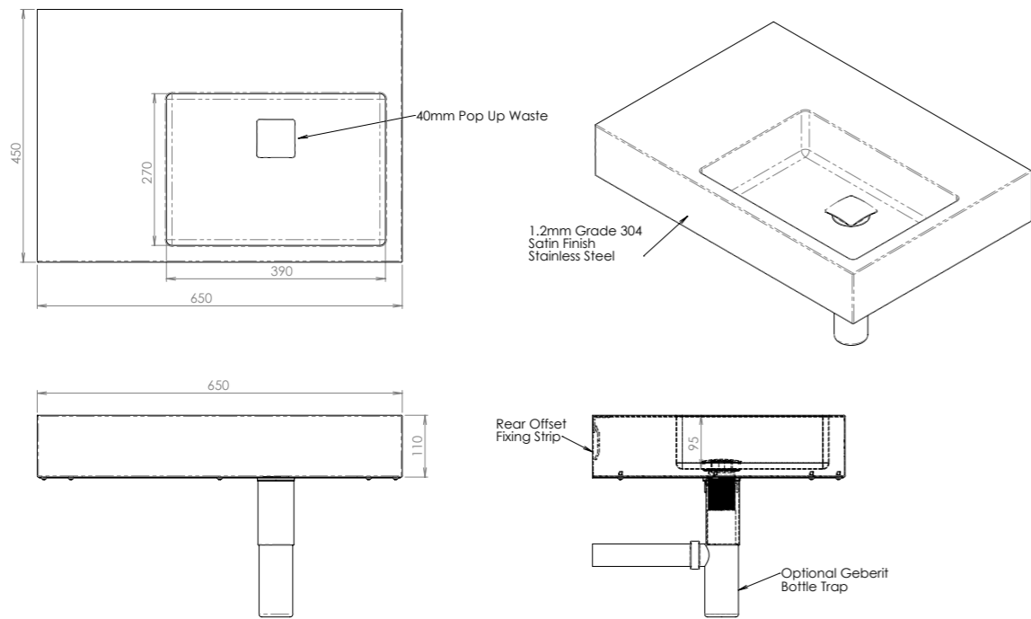
Fig 1: HBBEL-D Drawing
