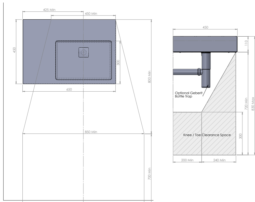
Fig 2: AS1428 Clearance Diagram
