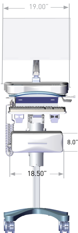
DRAWER DIMENSIONS
