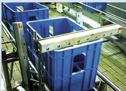
Three Model 110018 18" (457mm) Super Air Knives completely surround and blowoff crates so they can be loaded immediately.
