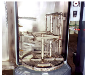
(3) Model 1212 12" (305mm) Standard Air Knives perform the drying cycle in this parts washer.
