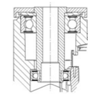
Double precision ball bearing
