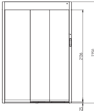
SLIDE SECUREDOOR VARIANT
