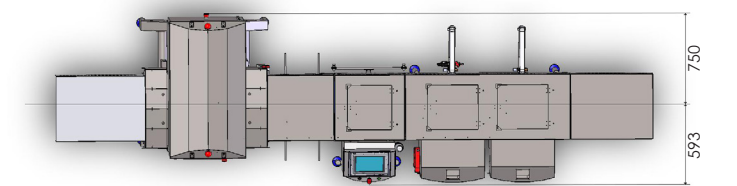
All measurements in mm (based on X5-500 with 400mm belt-width CW3)
