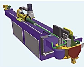
彎管虛擬 3D Simulation
