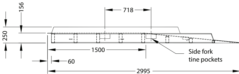
Popup fork slots which make it easy to move around with a forklift
