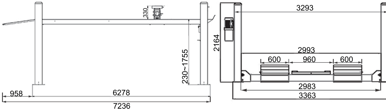
Turntable Recesses With Filler Plates (Turntables not included)
