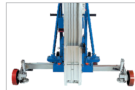
GL-850DC with front legs extended
