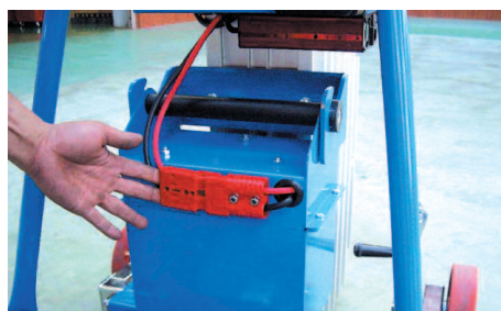
The battery on DC units is protected by a steel housing and is easily connected with a plug.
