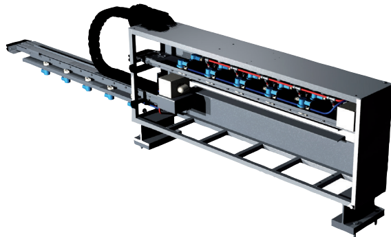
➤ spray.xact c: The spraying nozzles are installed on a telescopic spray bar with a cable and hose carrier in a housing.
