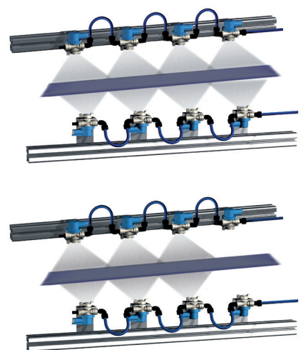
› spray.xact b : The perfect solution for oiling blanks or coils. The spraying nozzles are mounted on a profile. Every nozzle can be adjusted individually to match the requirements of the surface that is to be sprayed.
