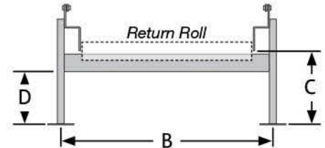
Intermediate Stand
