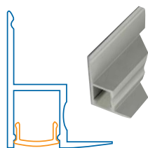
Recessed Ceiling Strip Light
