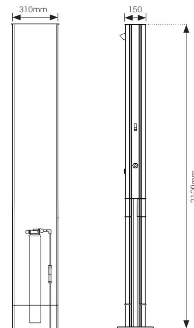
Front & side view showing optional filter detail
