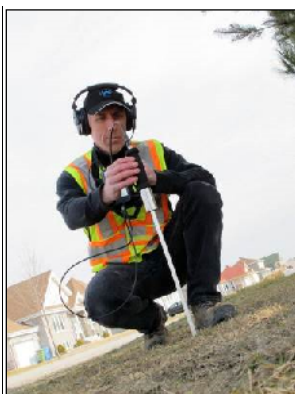
Fig.3 listening directly on a pipe with the rod inserted through soft soil -Not Recommended
