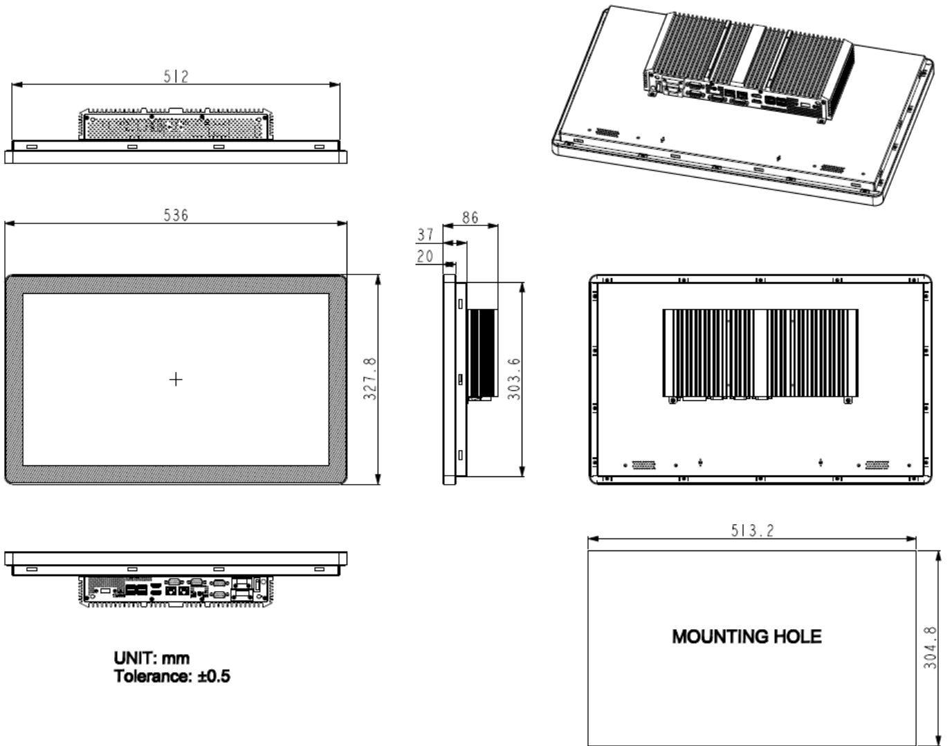
Figure 1.1: Dimensions of NPP-215P01
