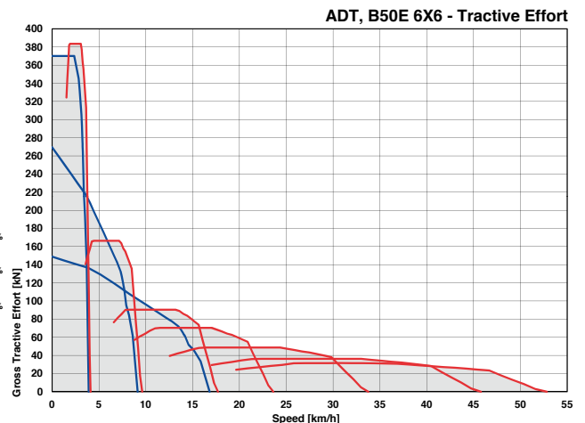
ADT, B50E 6X6 - Tractive Effort
