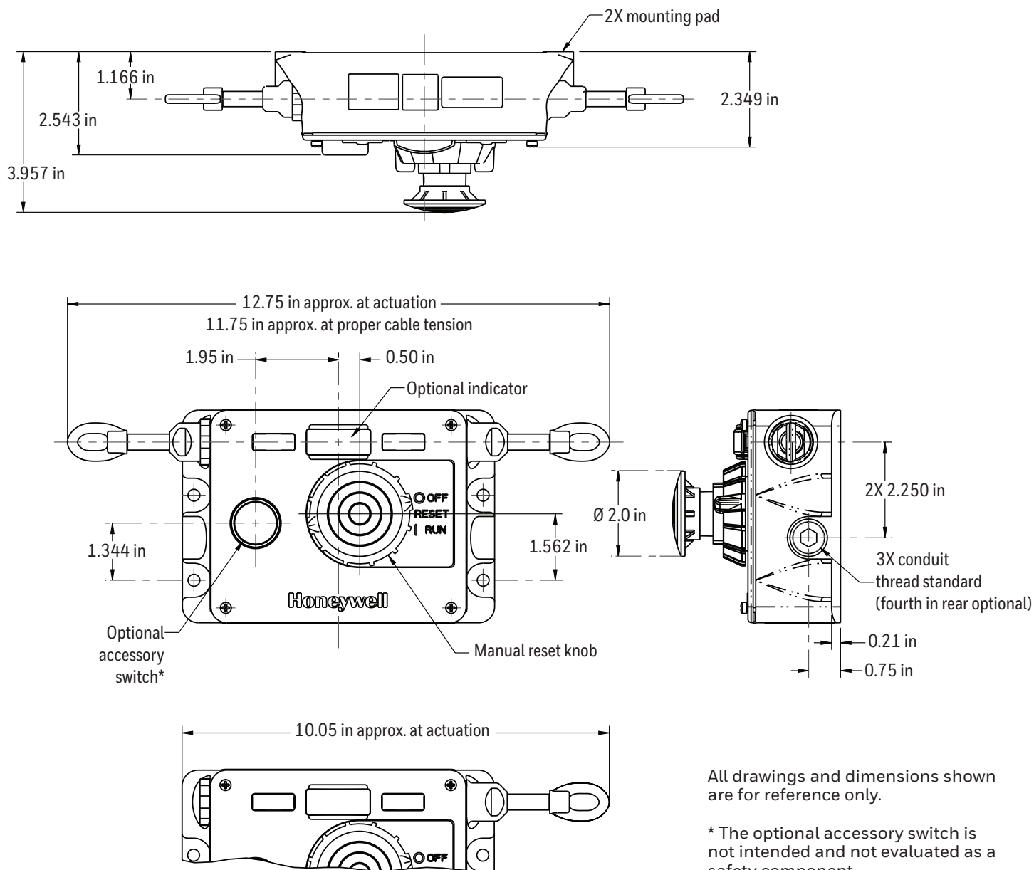
FIGURE 2. MOUNTING DIMENSIONS
