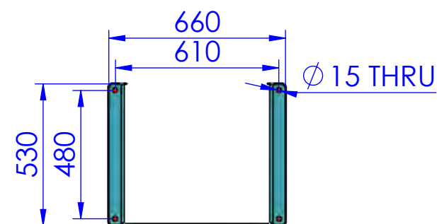
ANCHORING HOLE FLOOR MODEL
