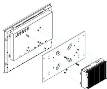
VESA Mount (Optional)
