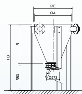
ANELLO SOTTOFILTRO A SALDARE FILTER MOUNTING UPSTAND
