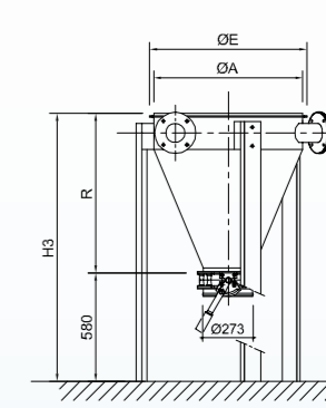
ANELLO SOTTOFILTRO A SALDARE FILTER MOUNTING UPSTAND
