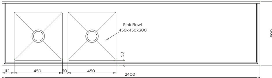
MODEL BT-DSB-624-L Plan
