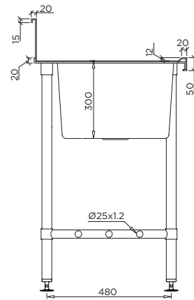
MODEL BT-DSB-618-L Section
