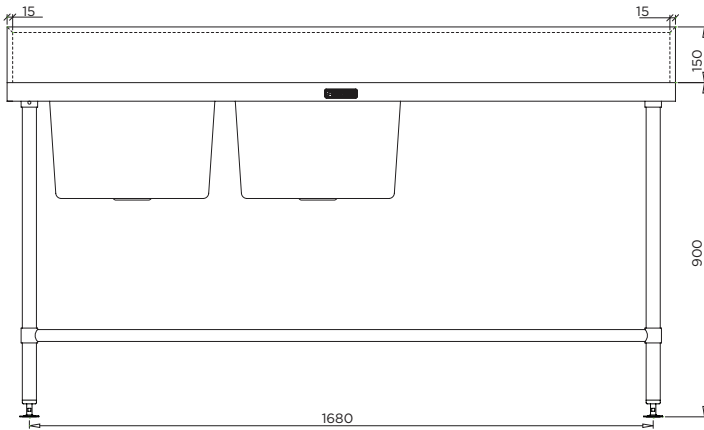
MODEL BT-DSB-618-L Front Elevation
