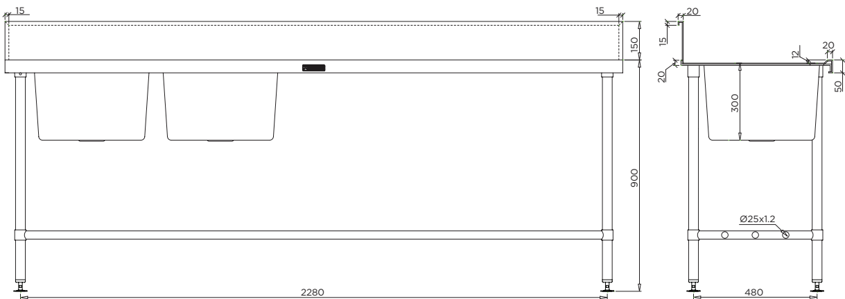
MODEL BT-DSB-624-L Front Elevation and Section
