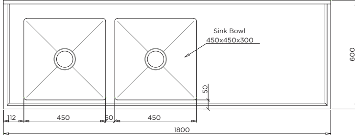
MODEL BT-DSB-618-L Plan
