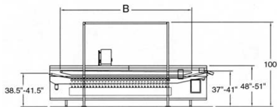
Elevation view
