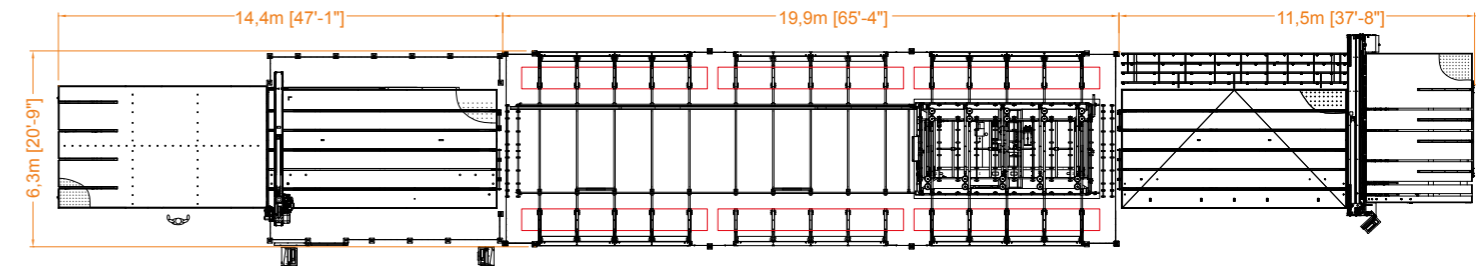
DISTRIBUTION 4: LT-06-MB + RUBI 406C + MT-600B4 + LAM 505S
