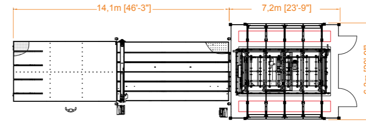
DISTRIBUTION 3: LT-06-FB + RUBI 306C + MT-600B4
