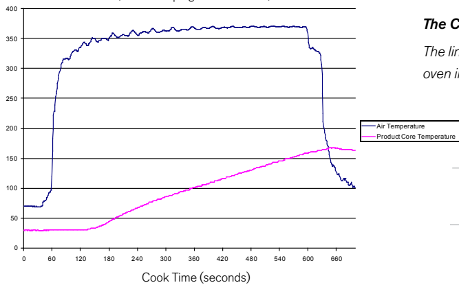
Product Core Temperature vs Air Temperature in GCO II (without Impingement Module)
