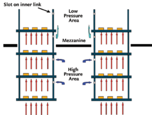
GCO II in Upflow Mode: Typical airflow patterns
