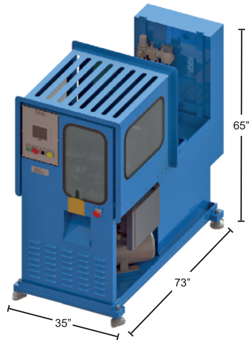
Model 1005HY Footprint 35"W x 73"D x 65"H
