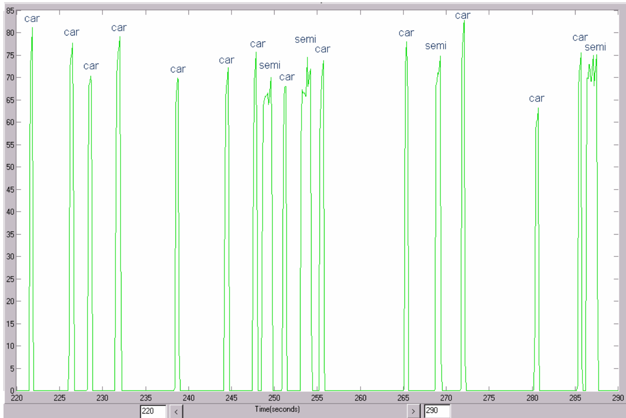
Figure 2 – Vehicle Speed (in MPH) vs. Time (in Seconds)
