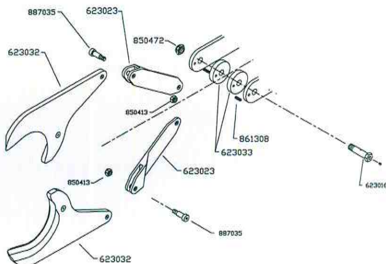
Figure 1 MODEL AHC – BLADE REPLACEMENT
