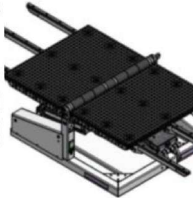
W-support arms for wider parts (EF-xW)
