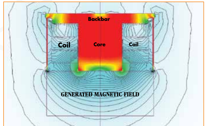
Finite element analysis and modeling a suspended electromagnet's magnetic field.
