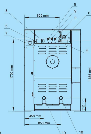
Rear side
