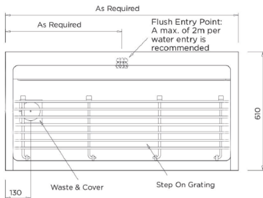
MODEL UREG Plan
