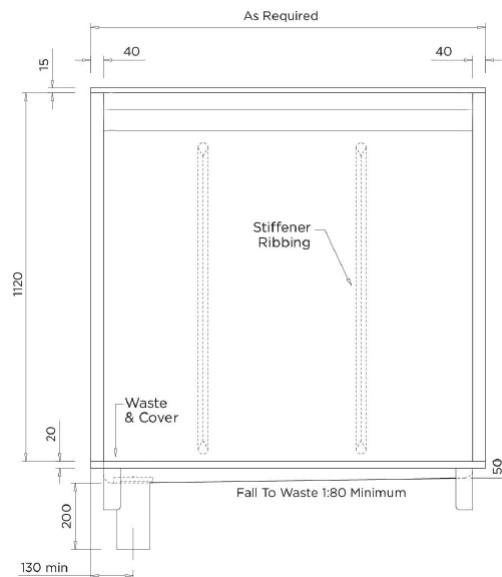
MODEL UREG Front Elevation
