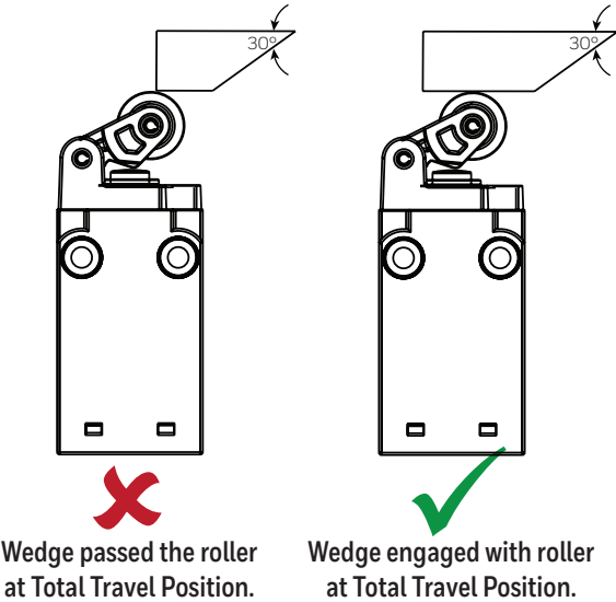
Figure 17. Wedge Actuation
